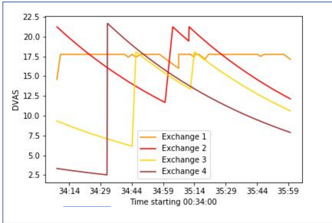
Figure 2: Decayed Volume Adjusted Scores Over Five-Minute Window From 34:00 to 35:00 Minutes After Midnight
